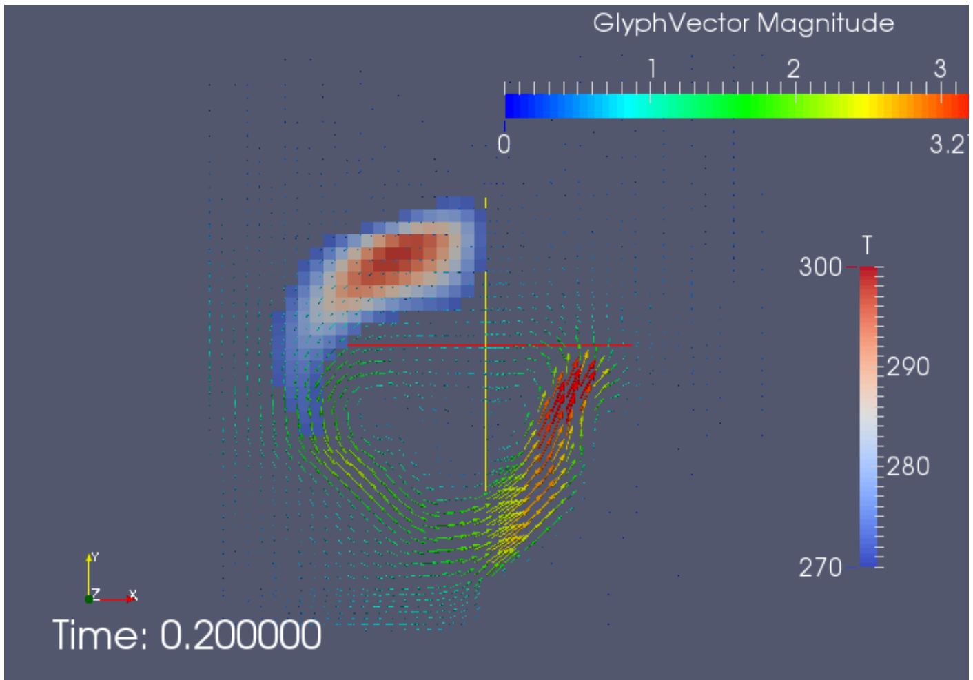
Figure: High-temperature region and velocity vector map
